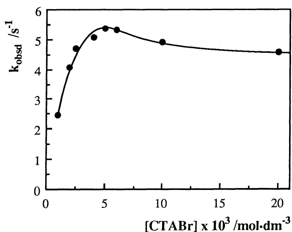
Fig. 1. Effect of CTABr concentration on the pseudo-first-order rate constants for the transacylation of PNPP at 25 °C, pH 7.03; [ 2 ]=[ \text{Cu}^{2+} ]= 1 \times 10^{-4} mol dm -3 , [ PNPP ]= 5 \times 10^{-5} mol dm -3 .
